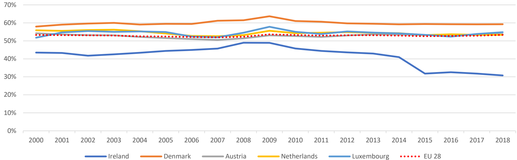
Labour Share by Country, 2000 -18
